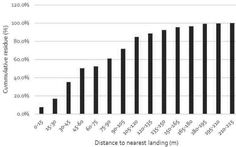
Figure 6.—Cumulative residue by distance from the landing in Washington ground-based harvest units.
