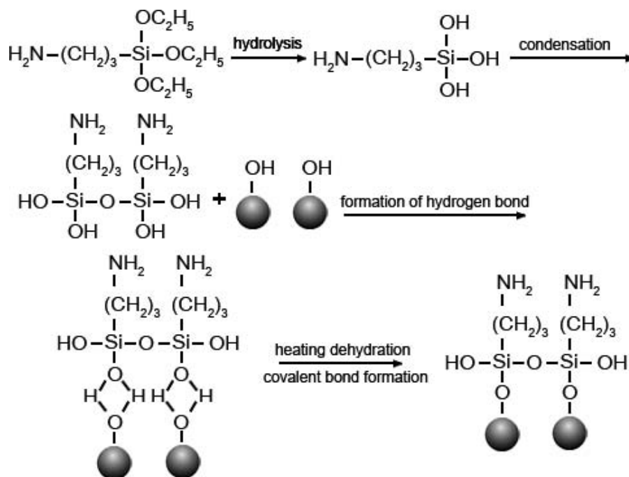
Figure 2.—Diagram of grafting KH-550 on nano-TiO 2 particle surface.
