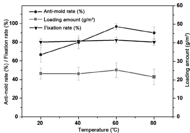
Figure 4.—Effect of reaction temperature on wood antimold rate, loading amount, and fixation rate (KH-550 concentration, 5 wt%; nano Ag/TiO 2 concentration, 1 wt%; incubation time, 2 h).
