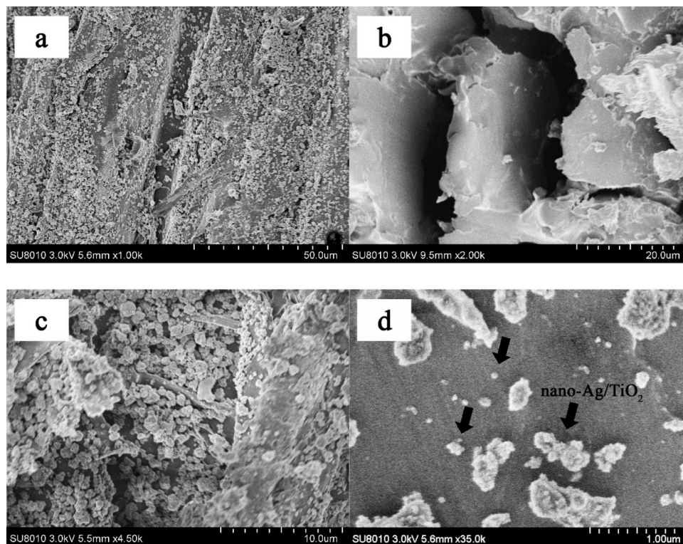
Figure 6.—Field emission scanning electron microscopy image of dispersion of modified nano-Ag/TiO 2 in Masson pine wood: radial sections (a, c, and d) and cross section (b).
