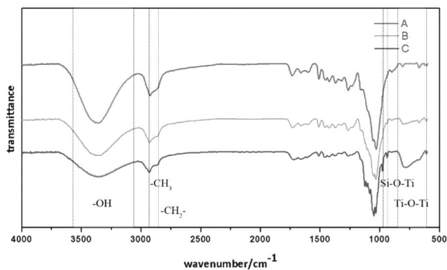
Figure 10.—Fourier transform infrared spectroscopy spectra of untreated wood (A), nano-Ag/TiO 2 -treated wood (B), and modified nano-Ag/TiO 2 -treated wood (C).
