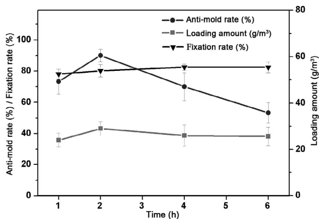
Figure 5.—Effect of incubation time on wood antimold rate, loading amount, and fixation rate (KH-550 concentration, 1 wt%; nano-Ag/TiO 2 concentration, 1 wt%; reaction temperature, 80°C).
