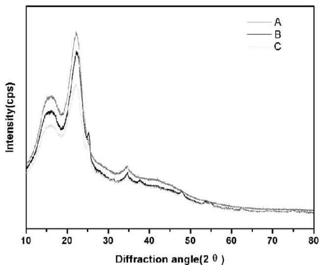
Figure 8.—X-ray diffraction spectra of untreated wood (A), nano-Ag/TiO 2 -treated wood (B), and modified nano-Ag/TiO 2 -treated wood (C).
