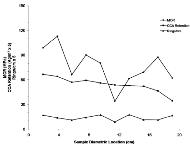
Figure 4.—Modulus of rupture, CCA retention, and ring density (rings per centimeter) of decommissioned utility Pole 1 at 5.6 m below the top (16 y in service).
